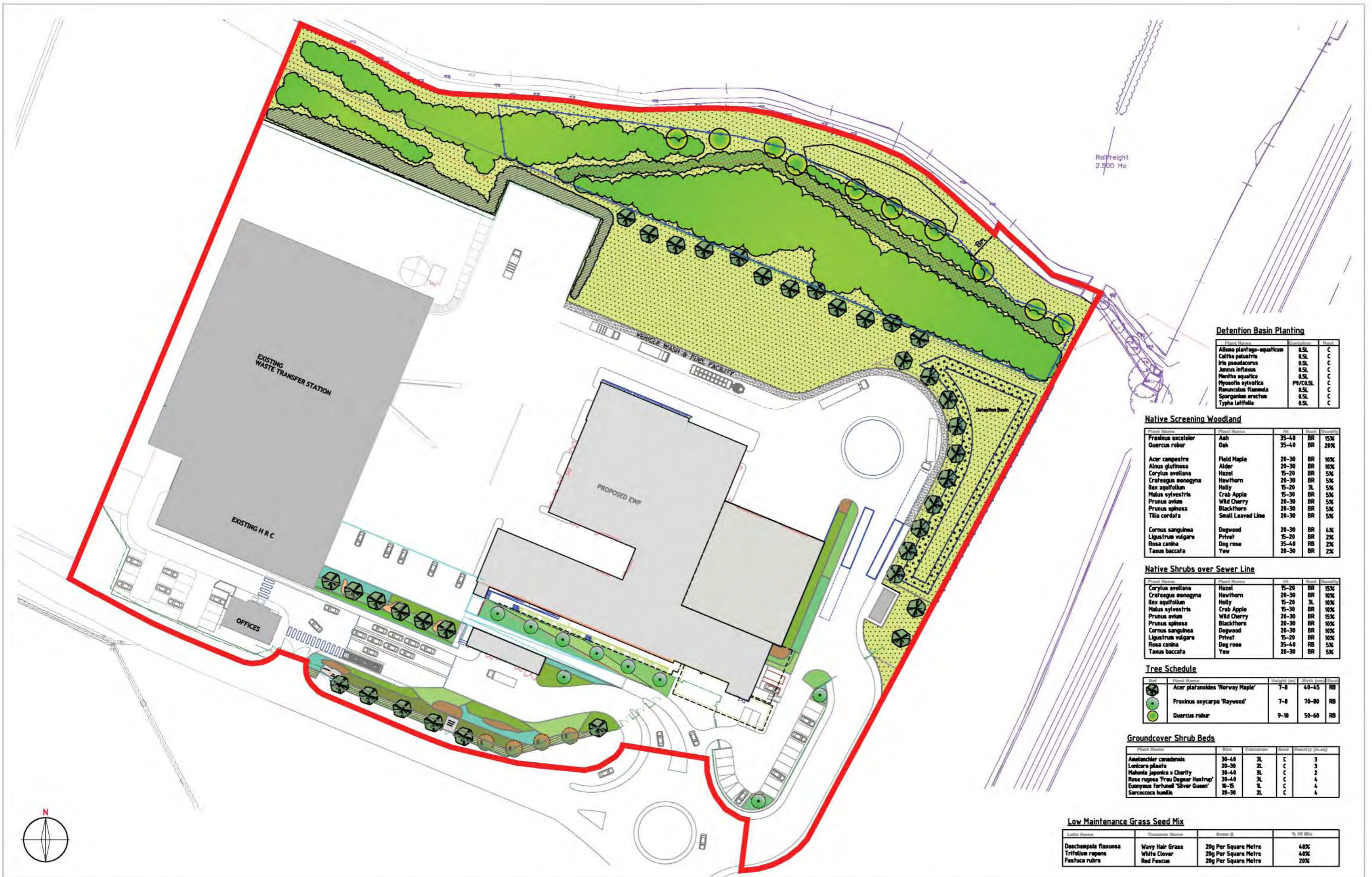
ENERGY FROM WASTE FACILITY BATTLEFIELD ENTERPRISE PARK SHREWSBURY FIGURE 4.1 INDICATIVE LANDSCAPE MASTERPLAN
